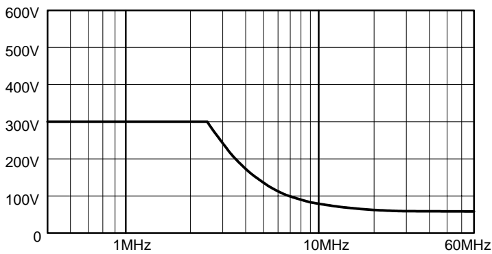
Figure 2: Maximum Working Voltage Derating Curve (V RMS )
